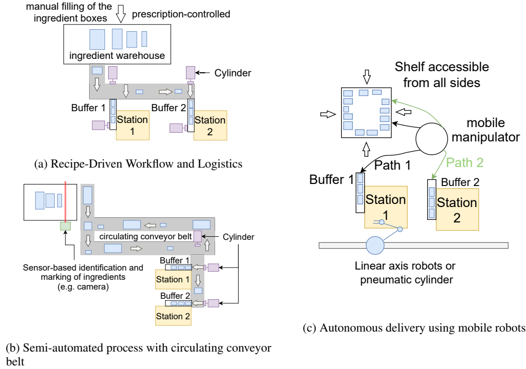
Figure 1: Concepts for the automation of large-scale kitchen environments with the goal of supporting cooking stations with ingredients at the recipe -defined correct sequence and timing.
